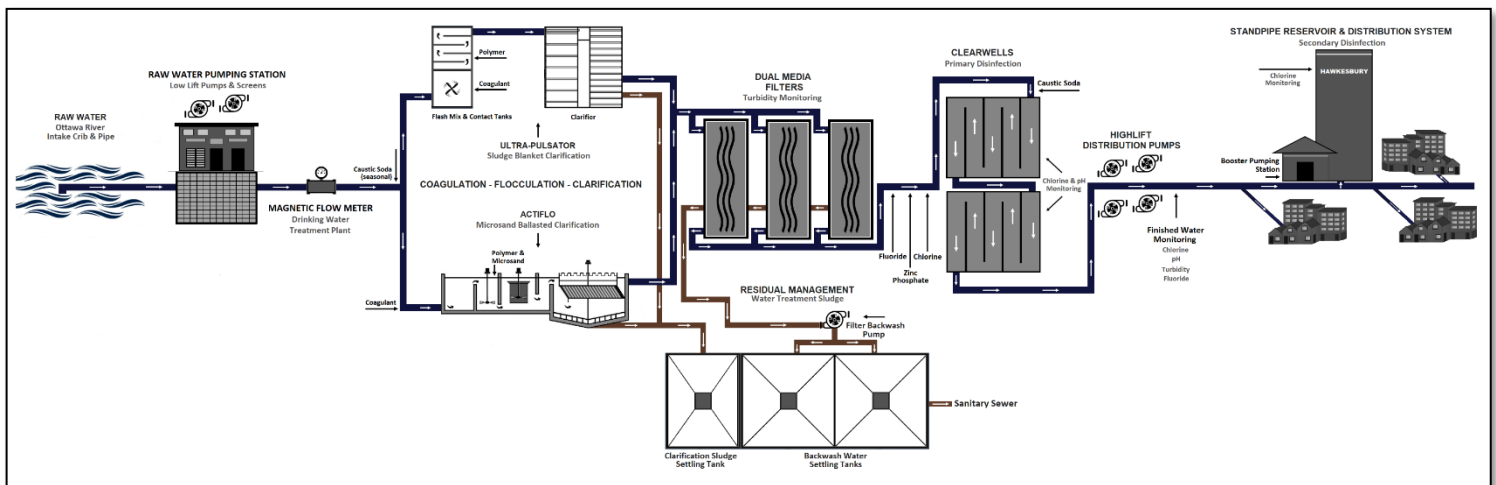
This process flow diagram is for reference only and represents a high-level overview of the system.
